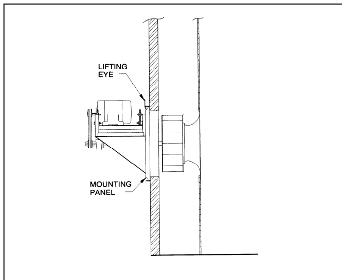
Figure 1 Typical Plug Fan Installation
